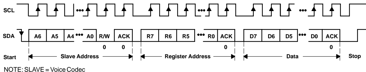
Figure 1. I 2 C Bus Write to Voice Codec
