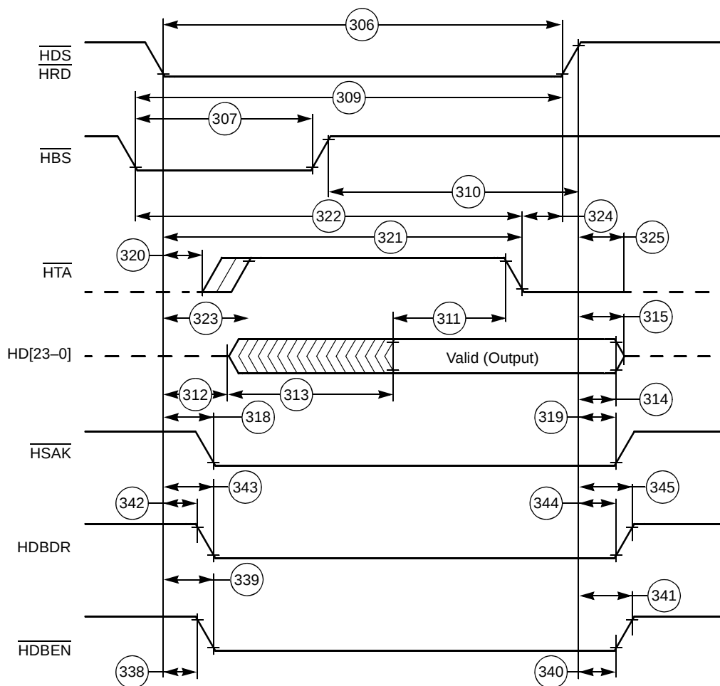
Figure 2-32. Read Timing
