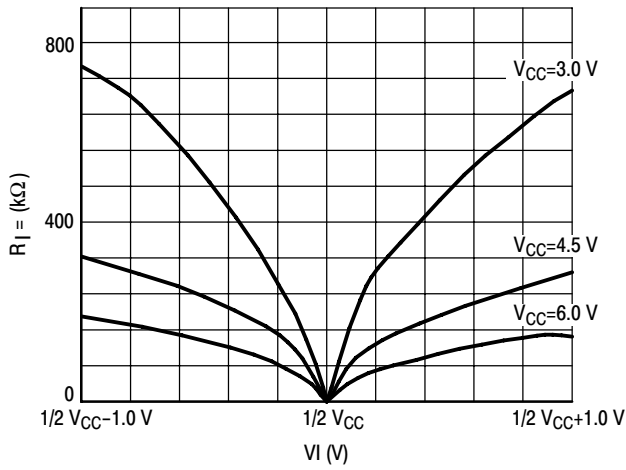
Figure 11. Input Resistance at SIG IN , COMP IN with \Delta V_I = 1.0 V at Self-Bias Point
