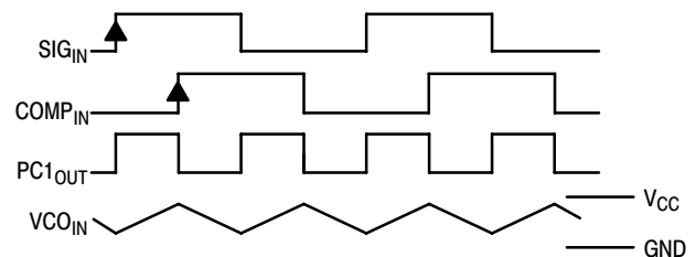
Figure 8. Typical Waveforms for PLL Using Phase Comparator 1
