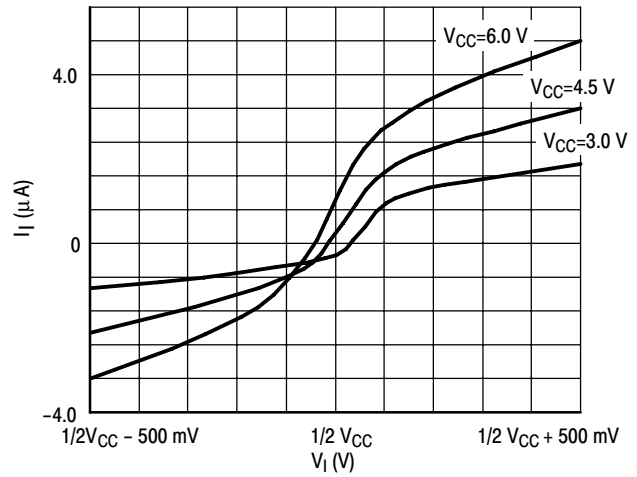
Figure 12. Input Current at SIG IN , COMP IN with \Delta V_I = 500 mV at Self-Bias Point
