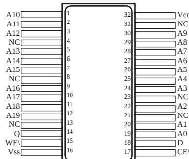
32-Pin Flat Pack (F)
