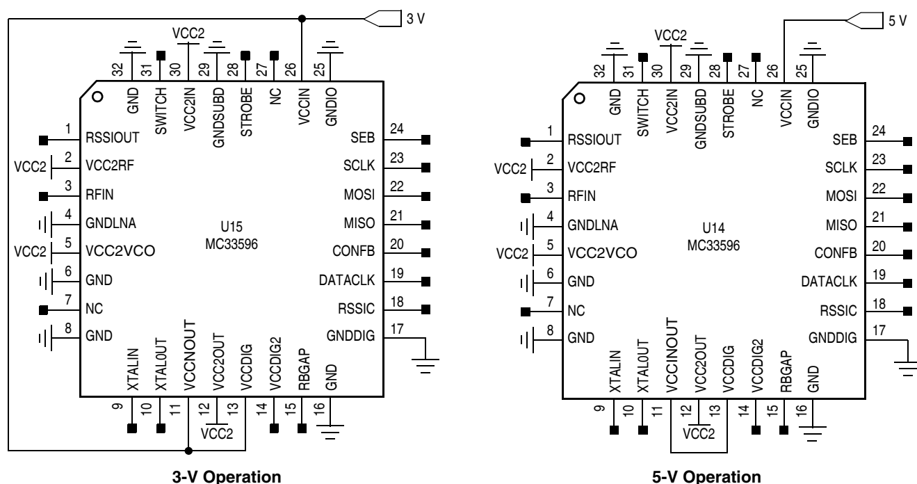
Figure 2. Wiring Diagrams
