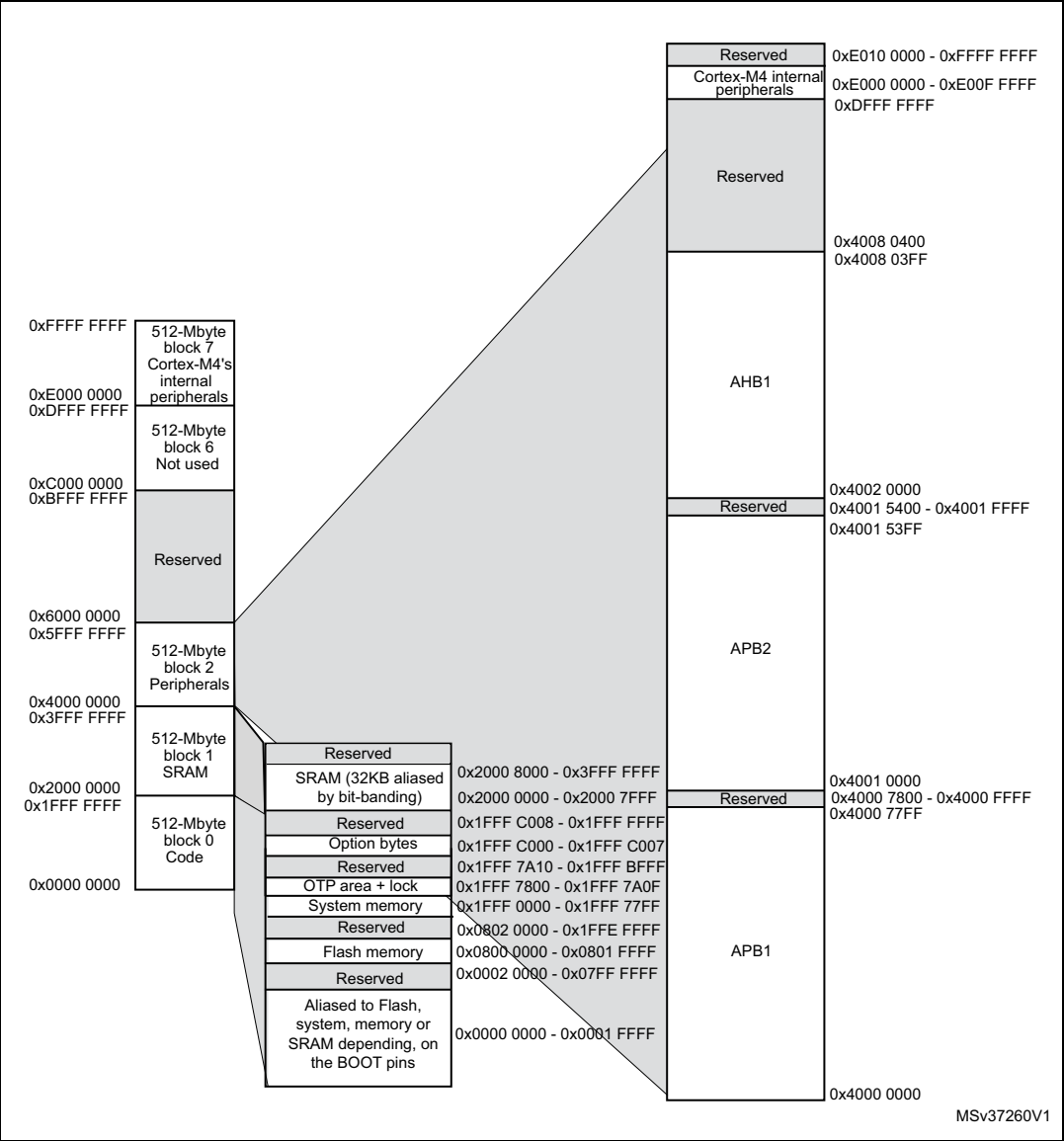
Figure 10. Memory map
