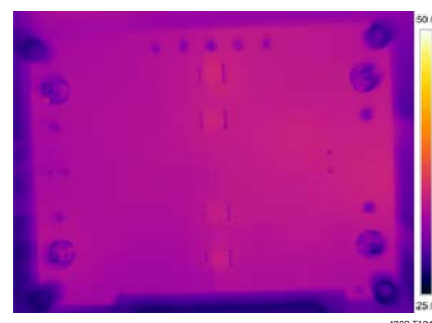
Thermograph of LT4320 Driving Four MOSFETs
