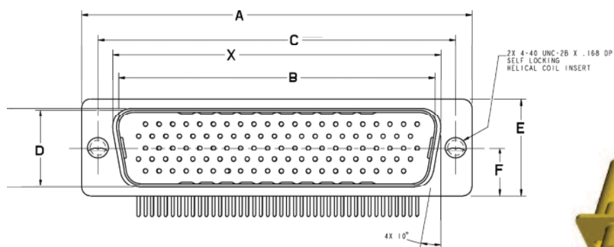
Plug - Pin
