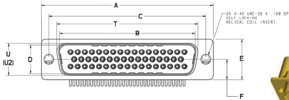
Plug - Pin
