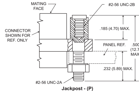
Jackpost - (P)
