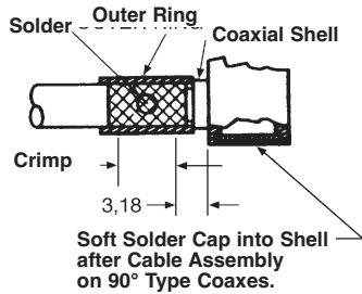
90° Coaxial
