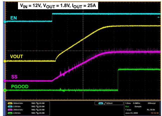
FIGURE 3. SOFT-START
