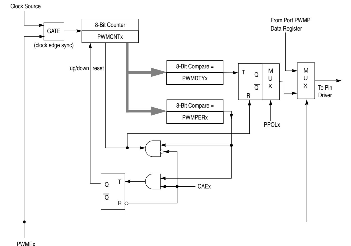
Figure 10-35. PWM Timer Channel Block Diagram
