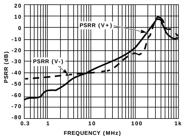
FIGURE 12. EL4342 PSRR CHANNELS A, B, C
