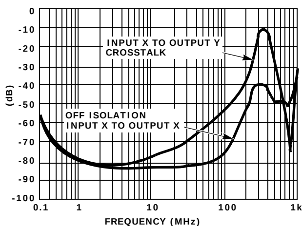
FIGURE 10. EL4342 CROSSTALK AND OFF-ISOLATION
