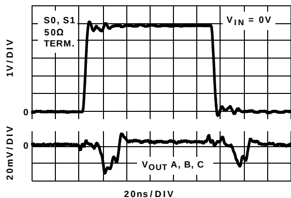
FIGURE 13. CHANNEL TO CHANNEL SWITCHING GLITCH V_{IN} = 0V
