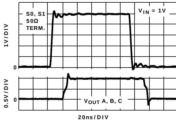
FIGURE 14. CHANNEL TO CHANNEL TRANSIENT RESPONSE V_{IN} = 1V
