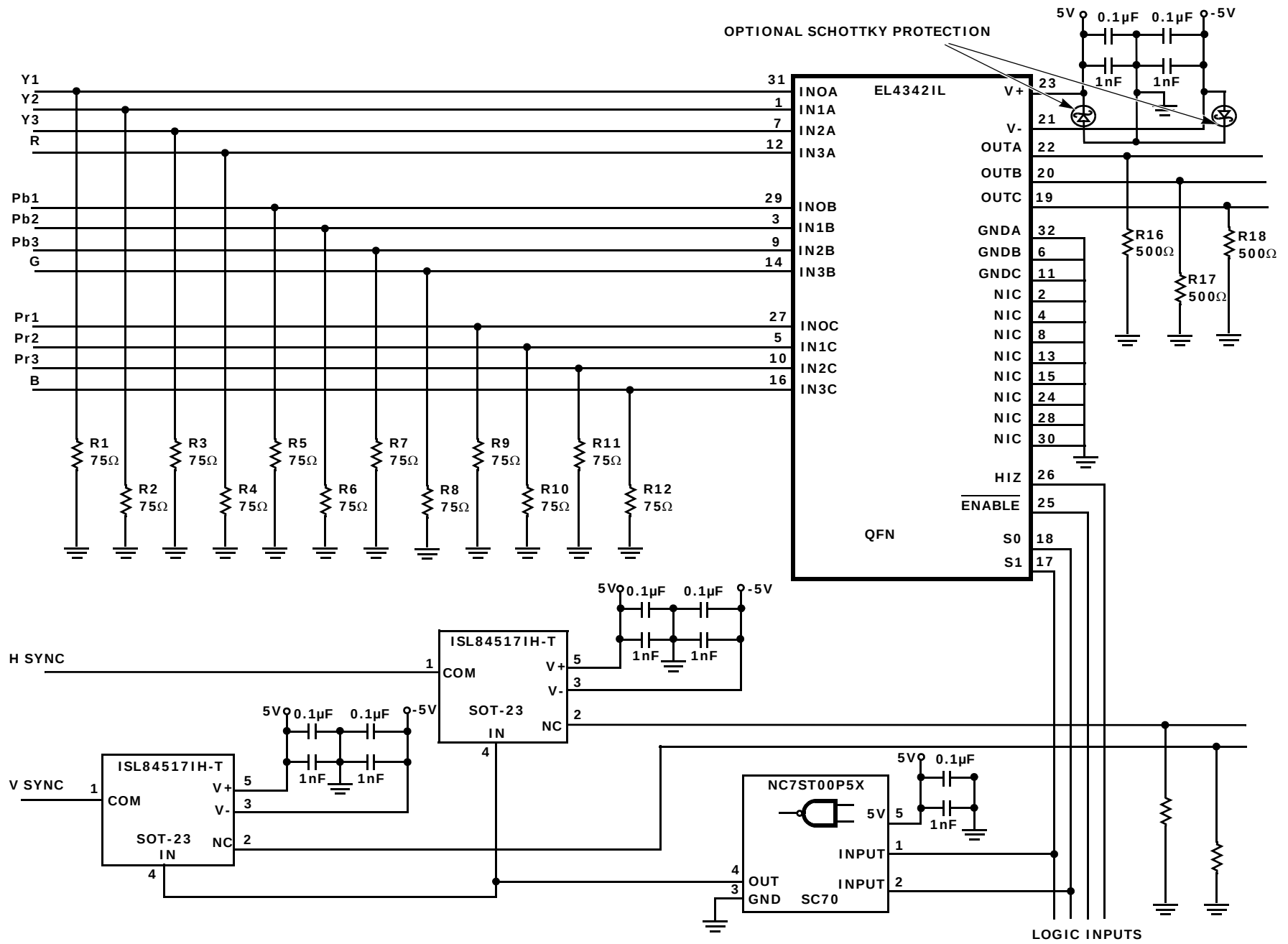
FIGURE 24. APPLICATION SHOWING THREE YPBPR CHANNELS AND ONE RGB+HV CHANNEL
