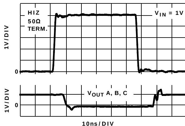
FIGURE 18. HIZ TRANSIENT RESPONSE V_{IN} = 1V
