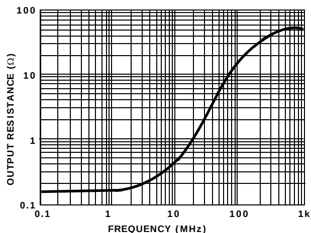
FIGURE 6. R_{OUT} vs FREQUENCY
