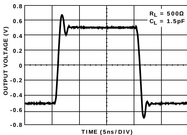
FIGURE 8. EL4342 TRANSIENT RESPONSE
