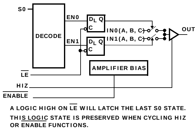
FIGURE 1. FUNCTIONAL DIAGRAM EL4340
