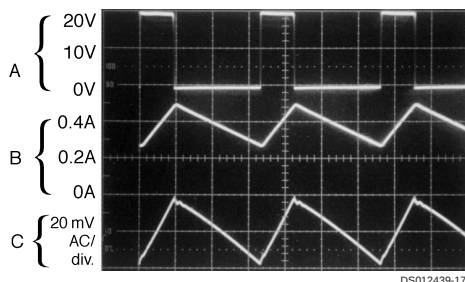
A: Output Pin Voltage, 10V/div. B: Inductor Current 0.2A/div. C: Output Ripple Voltage, 20 mV/div.
