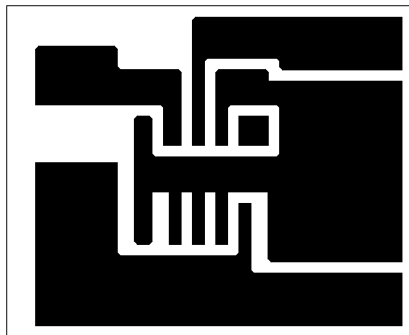
TYPICAL SURFACE MOUNT PC BOARD LAYOUT, FIXED OUTPUT (2X SIZE)
