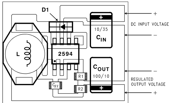
TYPICAL SURFACE MOUNT PC BOARD LAYOUT, ADJUSTABLE OUTPUT (2X SIZE)
