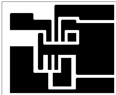
TYPICAL SURFACE MOUNT PC BOARD LAYOUT, ADJUSTABLE OUTPUT (2X SIZE)
