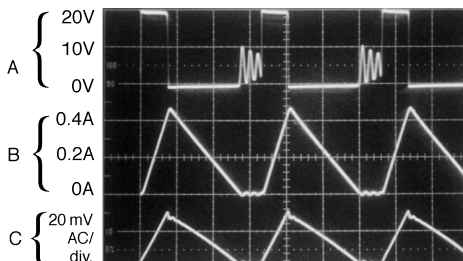
A: Output Pin Voltage, 10V/div. B: Inductor Current 0.2A/div. C: Output Ripple Voltage, 20 mV/div.
