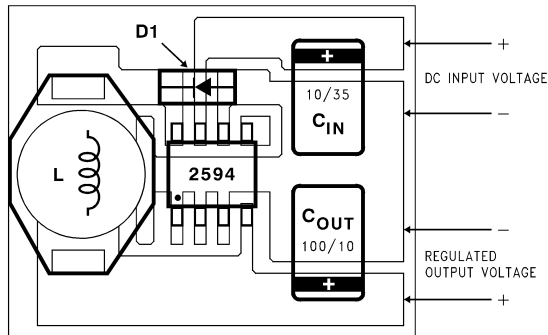
TYPICAL SURFACE MOUNT PC BOARD LAYOUT, FIXED OUTPUT (2X SIZE)
