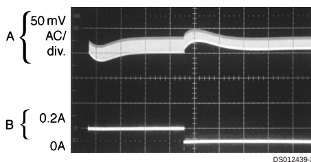
A: Output Voltage, 50 mV/div. (AC) B: 100 mA to 200 mA Load Pulse
