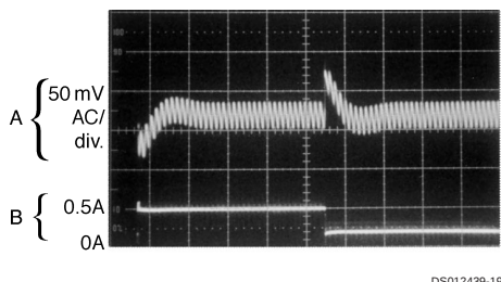
A: Output Voltage, 50 mV/div. (AC) B: 200 mA to 500 mA Load Pulse
