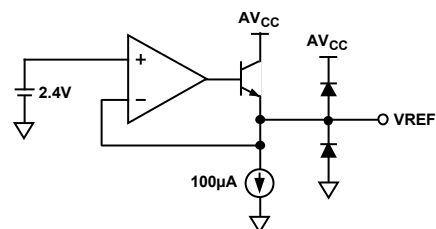
Figure 36. 2.4 V Reference
