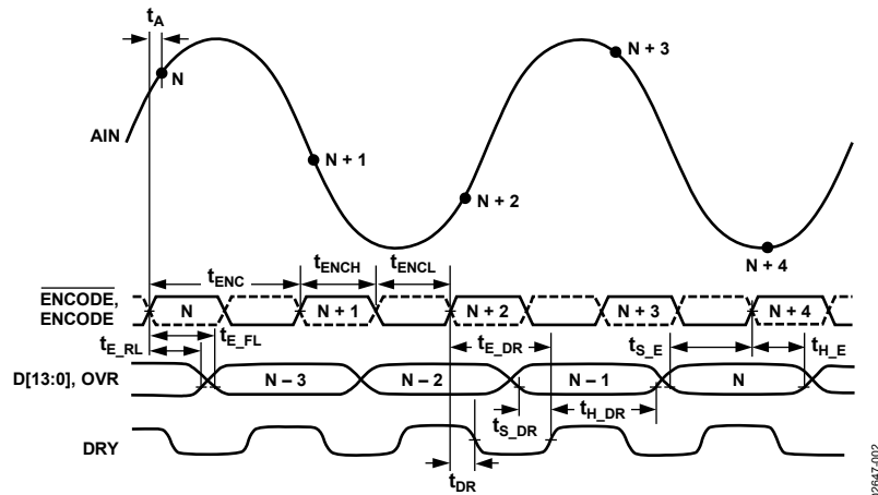
Figure 2. Timing Diagram
