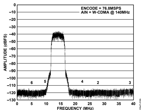
Figure 30. W-CDMA Tone @ 140 MHz, Encode = 76.8 MSPS
