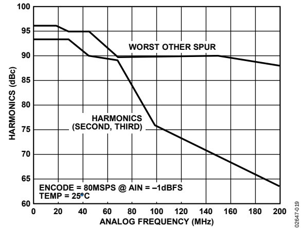
Figure 13. Harmonics vs. Analog Frequency (fF)
