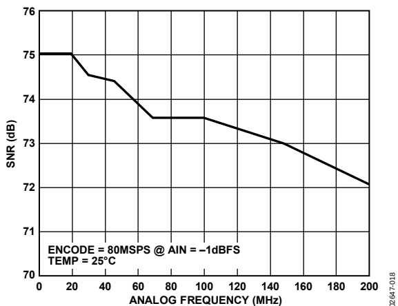
Figure 12. Signal-to-Noise Ratio (SNR) vs. Analog Frequency (fF)
