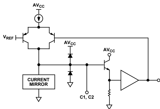
Figure 34. Compensation Pin, C1 or C2
