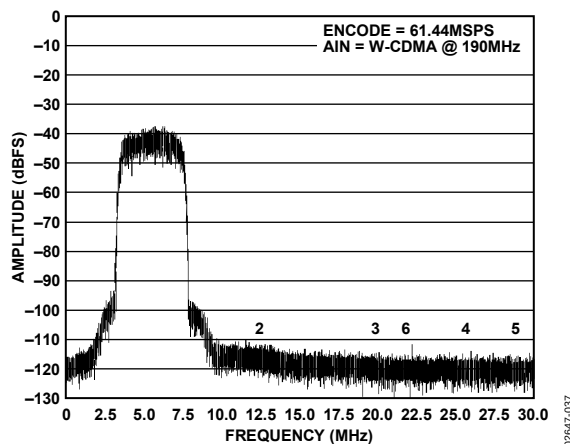
Figure 31. W-CDMA Tone @ 190 MHz, Encode = 61.44 MSPS
