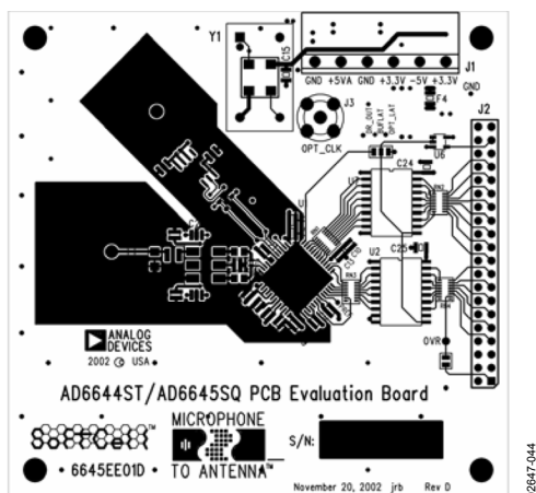
Figure 44. Top Signal Level
