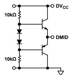
Figure 37. DMID Reference
