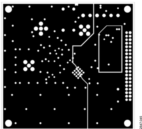
Figure 45. 5.0 V Plane Layer 3 and 3.3 V Plane Layer 4
