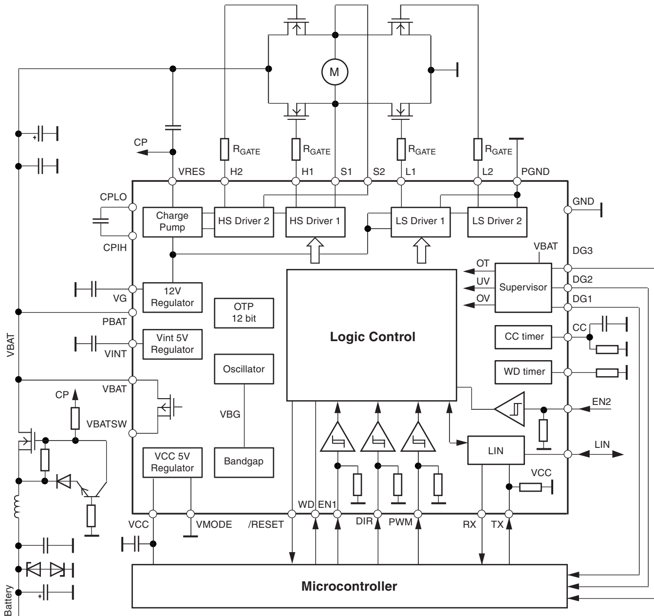
Figure 1-1. Block Diagram
