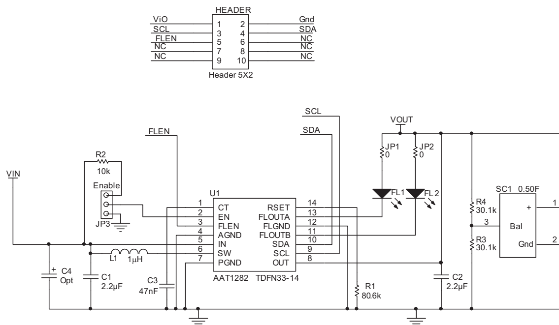
Figure 12: AAT1282 DB2 USB/I²C Evaluation Board Schematic.
