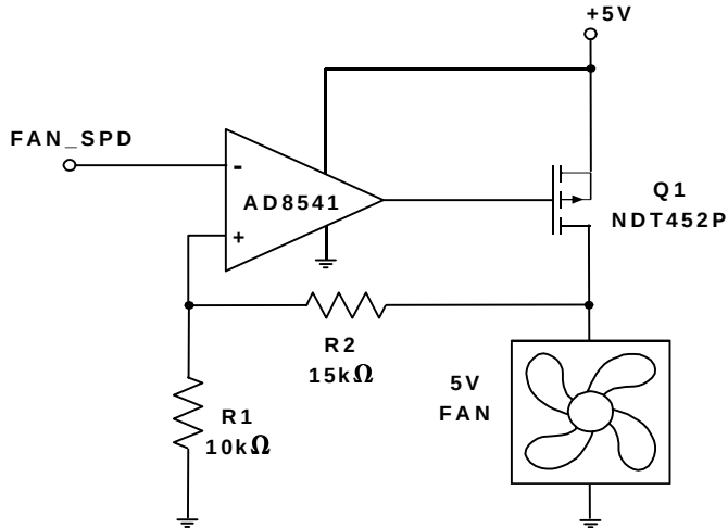
Figure 14a. 5V Fan Circuit with Op-Amp
