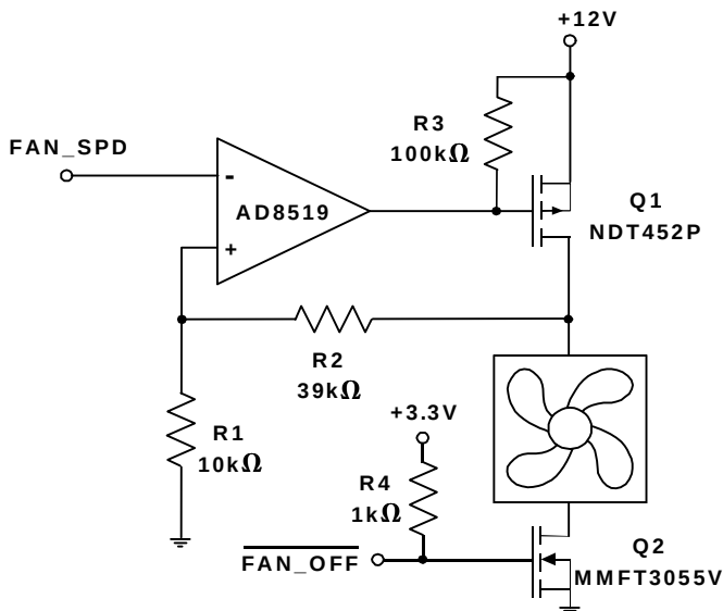
Figure 14c. 12V Fan Circuit with Op-Amp and P-Channel MOSFET
