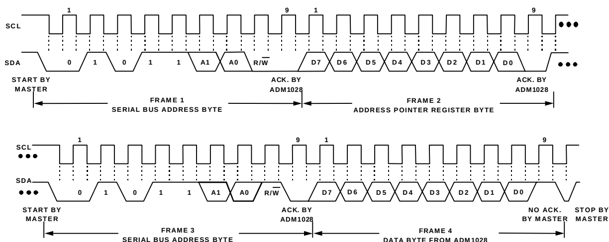
Figure 11b. Reading Data from the ADM1028
