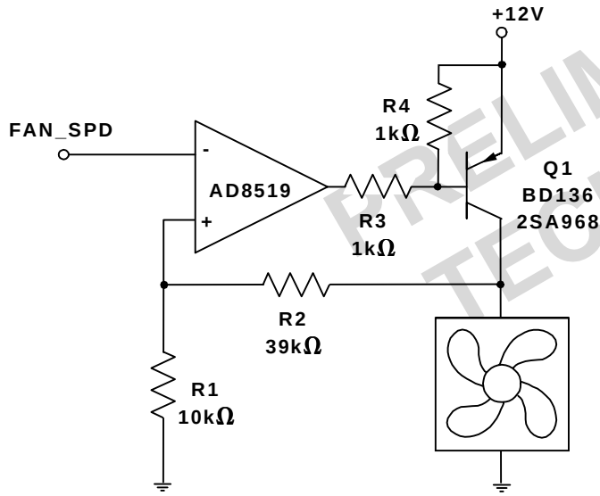
Figure 14b. 12V Fan Circuit with Op-Amp and PNP Transistor
