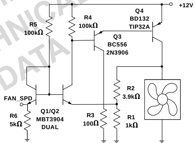
Figure 14e. Discrete 12V Fan Drive Circuit with Bipolar Output Single Supply
