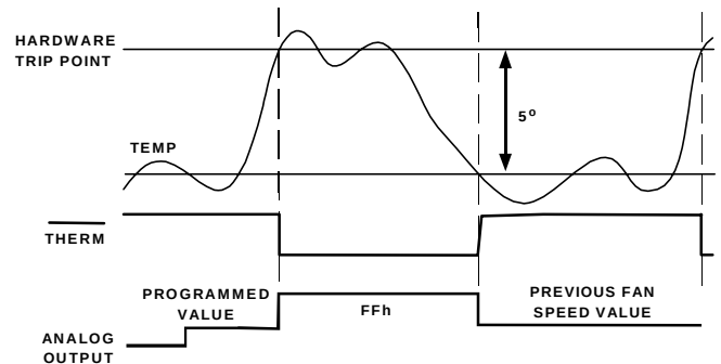
Figure 16. Operation of \overline{\text{THERM}} Outputs
