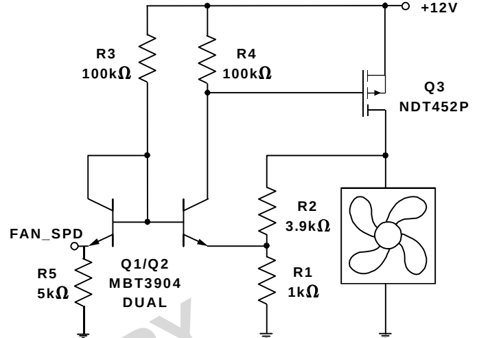
Figure 14d. Discrete 12V Fan Drive Circuit with P-Channel MOSFET, Single Supply
