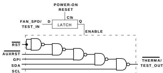
Figure 21. NAND Tree
