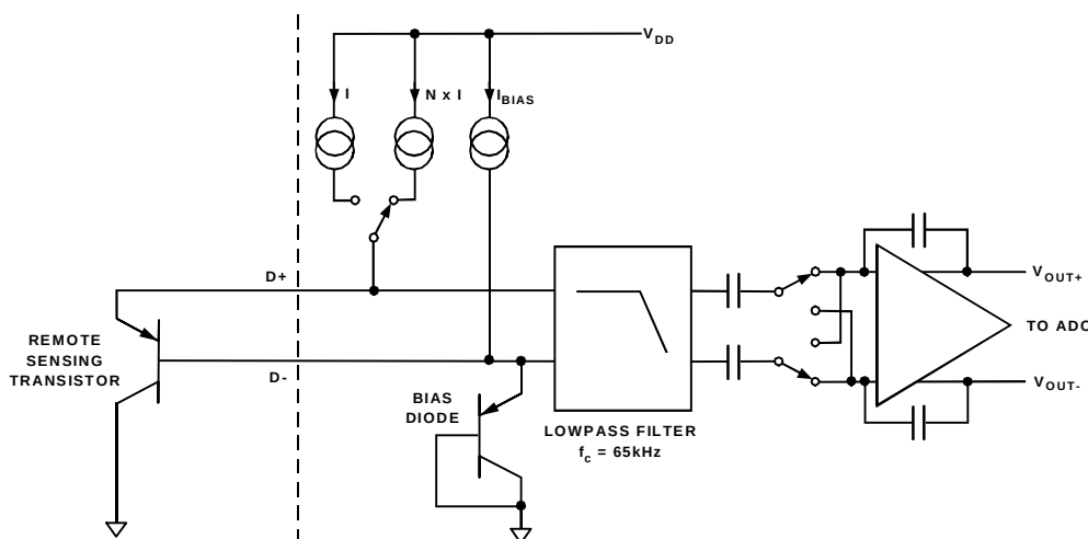
Figure 12. ADM1028 Signal Conditioning
