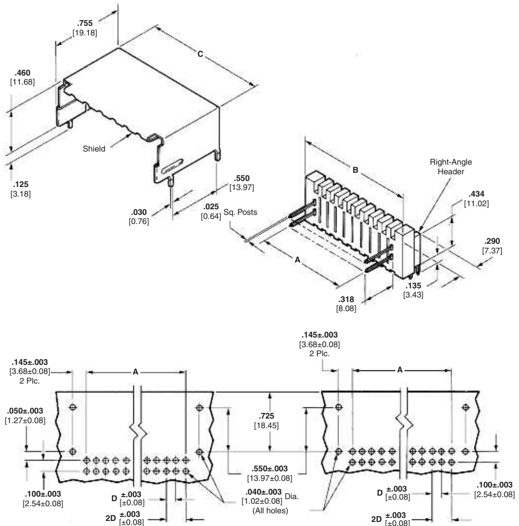
Recommended PC Board Hole Layout for 6, 8 and 10 Positions
