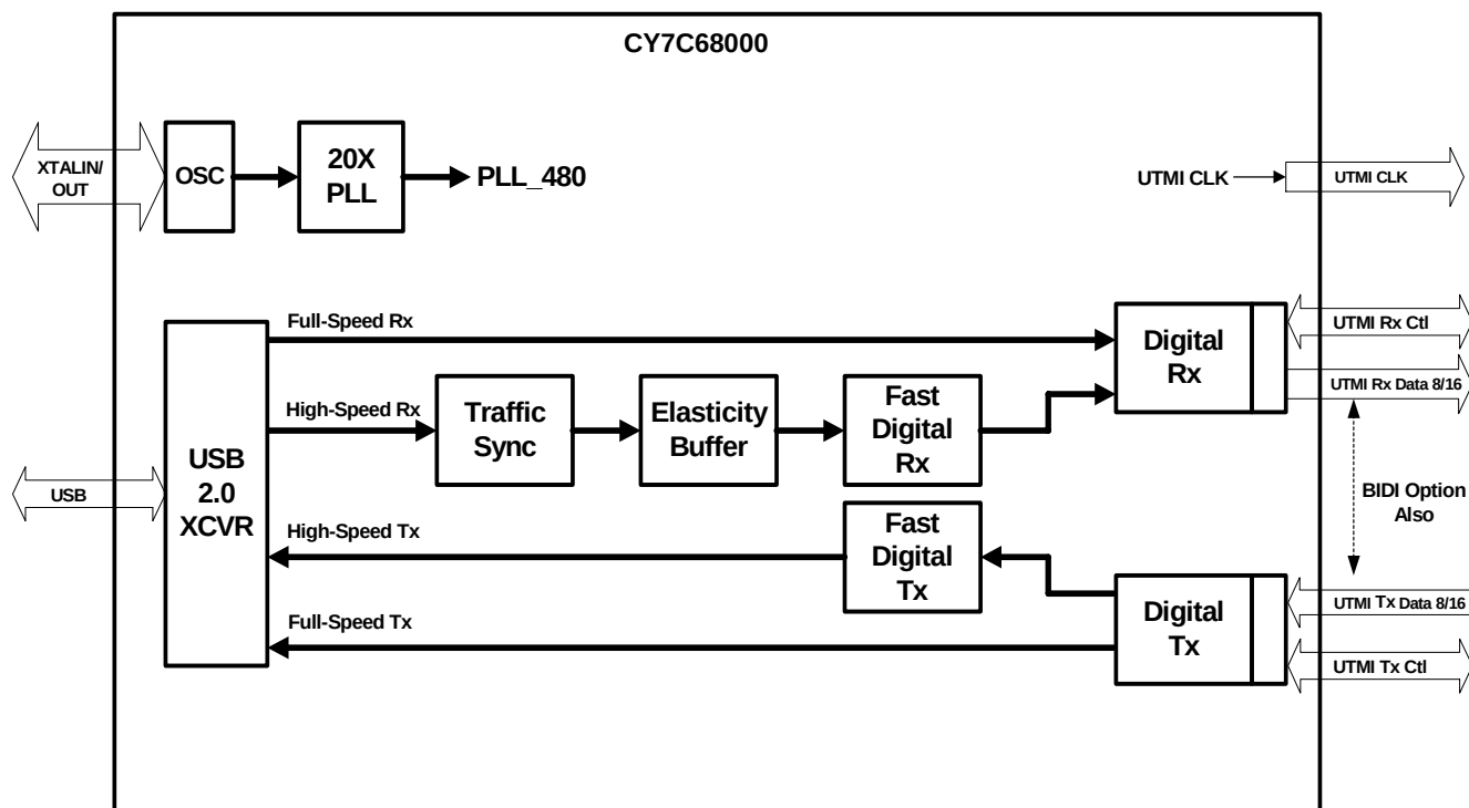
Figure 1-1. Block Diagram
