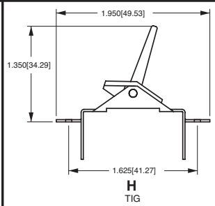
WIDE FW TIL, TIG, TIH, TII METAL, SNAP-IN
