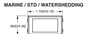
MARINE / STD / WATERSHEDDING MBL, NBL, WBL TIG BLACK NYLON, SNAP-IN
