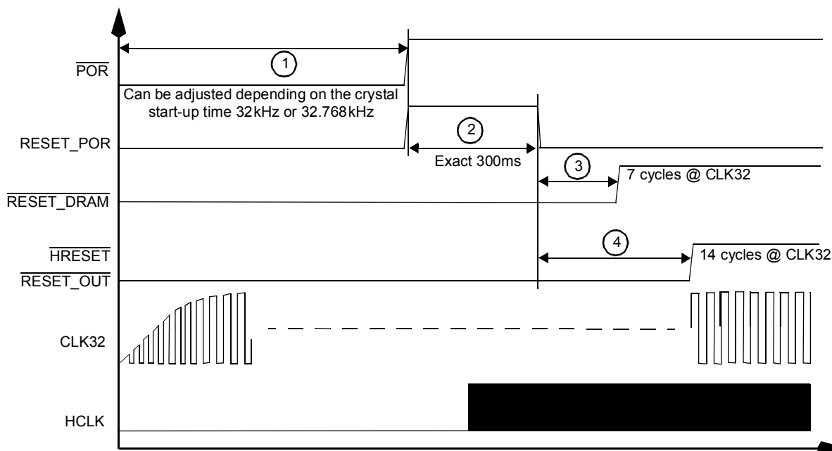
Figure 2. Timing Relationship with \overline{\text{POR}}
