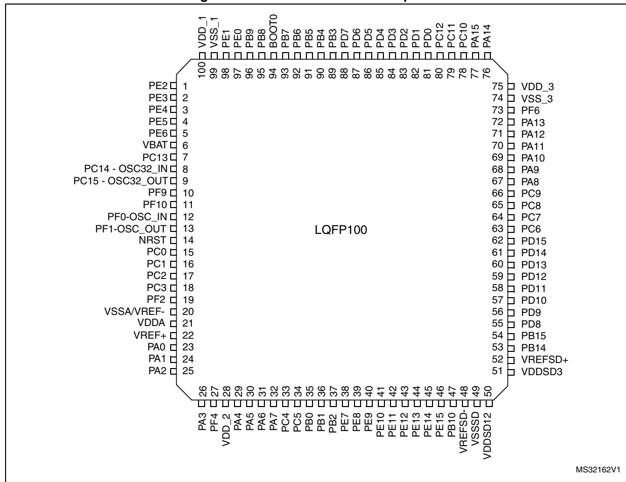
Figure 4. STM32F373xx LQFP100 pinout
