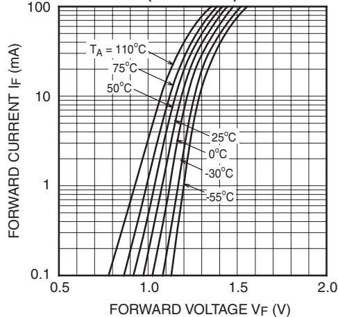
Fig. 5 Forward Current vs. Forward Voltage (FOD617/817)
