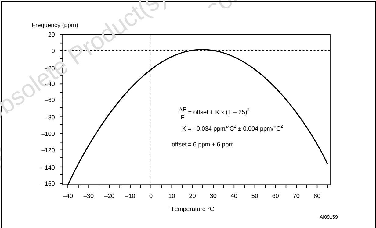
Figure 4. Crystal accuracy across temperature
