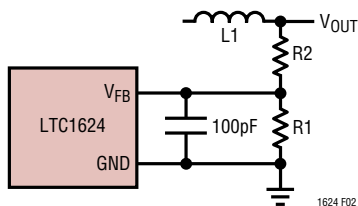
Figure 2. Setting the LTC1624 Output Voltage
