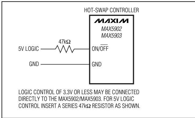
Figure 5. Logic Control
