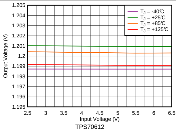
Figure 1. 1.2-V Line Regulation vs V_{\text{IN}} and Temperature
