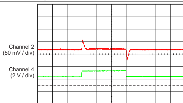
Channel 2 = V_{OUT} , channel 4 = V_{IN} , I_{OUT} = 50\text{ mA} Time (50 \mu\text{s} / div)
