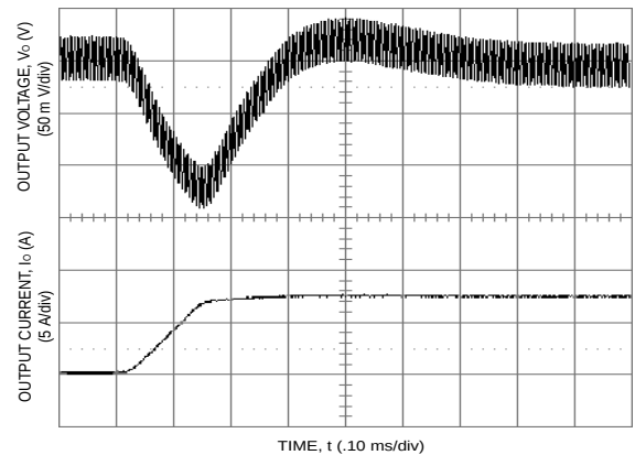
Figure 29. Transient Response to Step Increase in Load from 50% to 75% of Full Load ( V_I = 48 Vdc).
