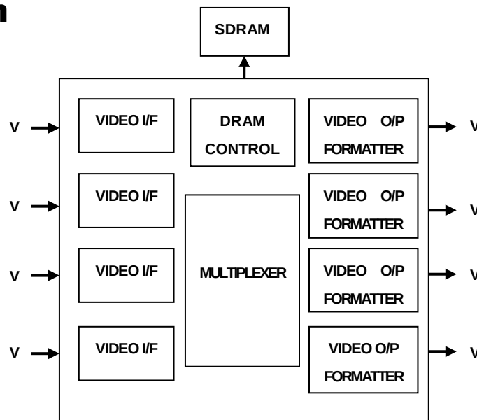
FIGURE 1. TW2826 BLOCK DIAGRAM
