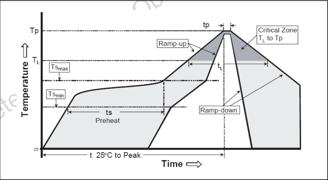
Figure 9. Soldering
