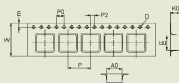
Tape Dimensions
