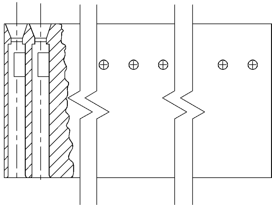
SECT Y-Y
