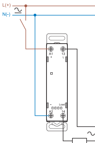
Connessione monofase (77.31.....7x)
