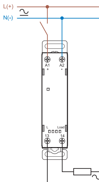
Connessione monofase (77.31.....5x)
