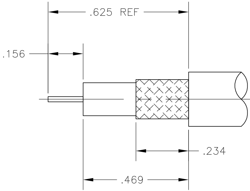
VIEW A
