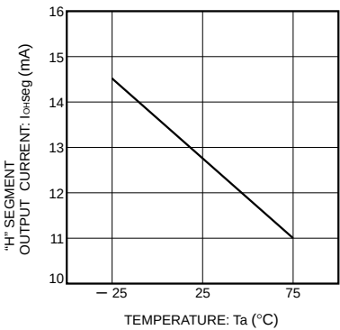
Fig.7 "H" segment output current temperature characteristics
