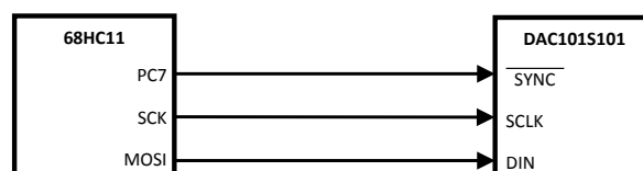
Figure 39. 68HC11 Interface
