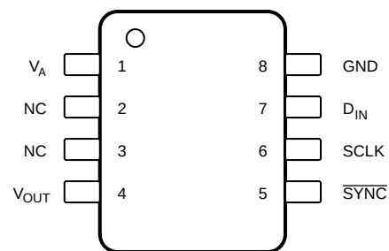
DAC101S101 DGG Package
