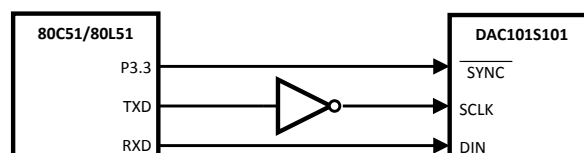
Figure 38. 80C51/80L51 Interface
