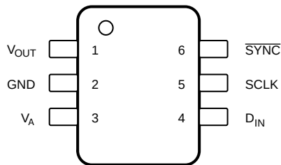
DAC101S101 and DAC101S101-Q1 DDC Package
