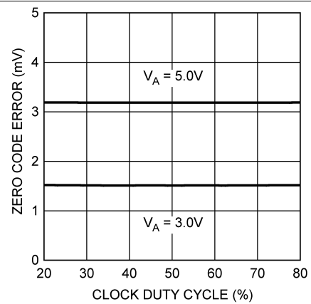
Figure 24. Zero Code Error vs. Clock Duty Cycle
