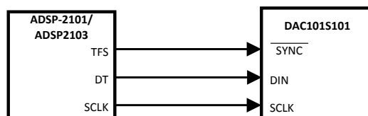
Figure 37. ADSP-2101/2103 Interface
