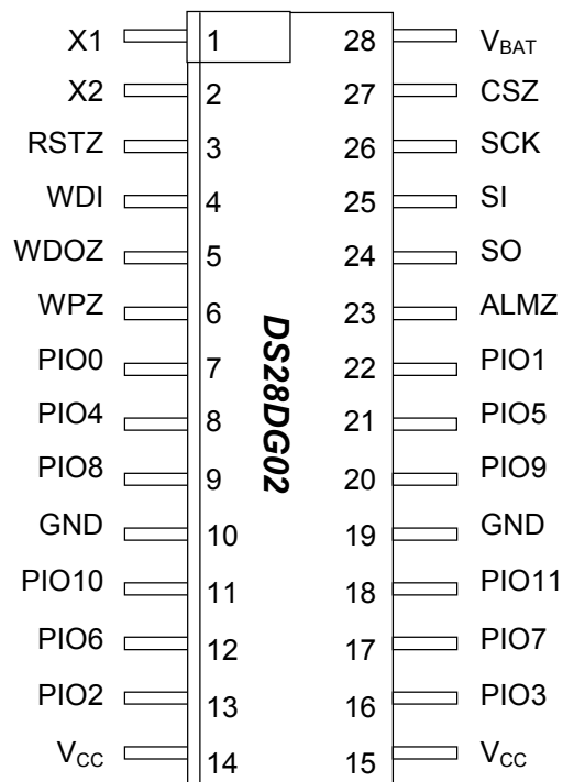
4.4mm 28-Lead TSSOP (Top View)
