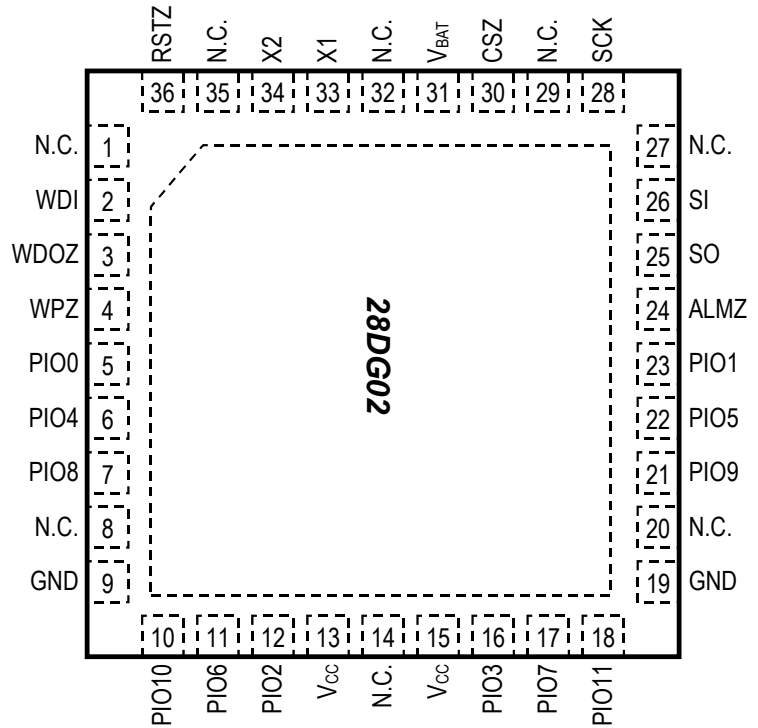
Thin 36-Lead 6mm x 6mm QFN (Top View)
