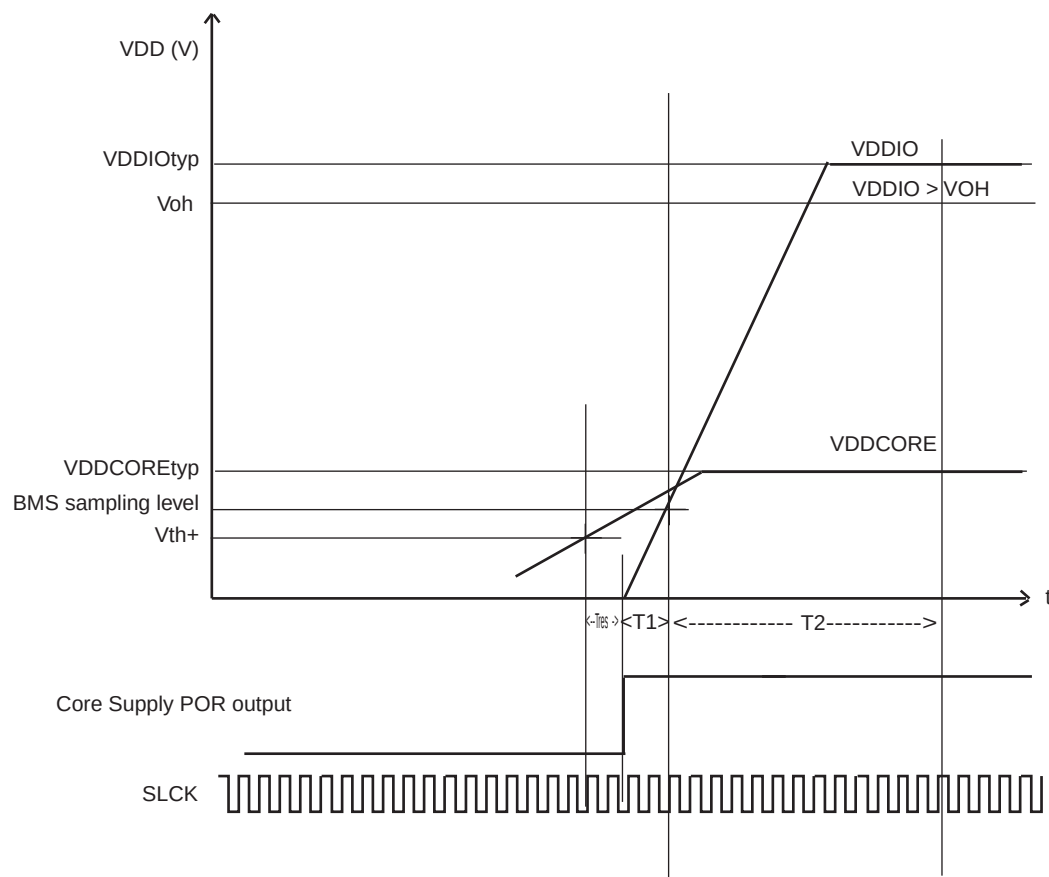
Figure 47-2. VDDCORE and VDDIO Constraints at Startup
