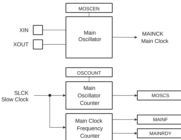
Figure 27-2. Main Oscillator Block Diagram
