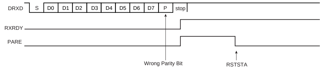
Figure 30-8. Parity Error
