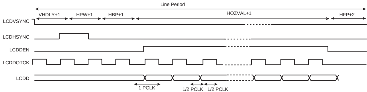
Figure 44-5. TFT Panel Timing (Line Expanded View), CLKMOD=1
