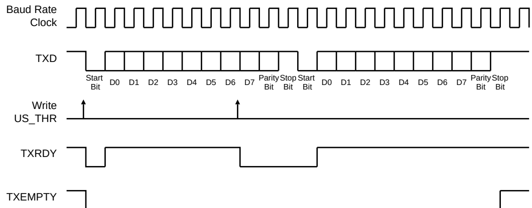
Figure 34-7. Transmitter Status
