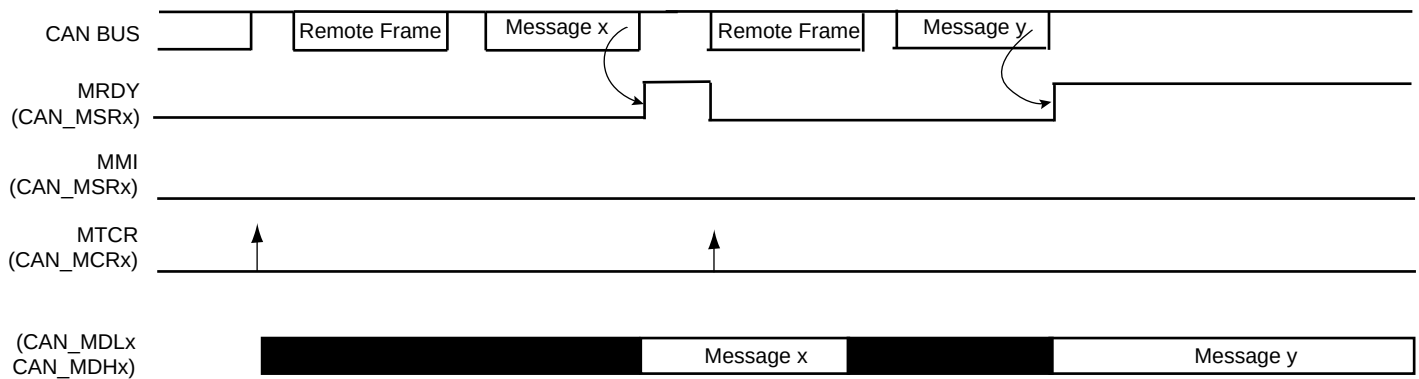
Figure 37-18. Consumer Handling
