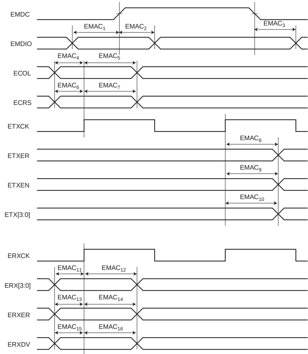
Figure 47-6. EMAC MII Mode
