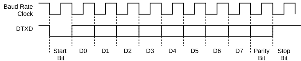
Figure 30-10. Character Transmission
