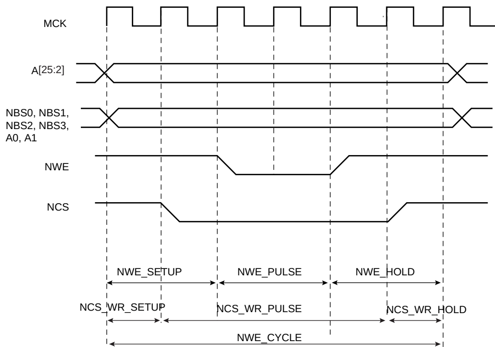
Figure 23-12. Write Cycle
