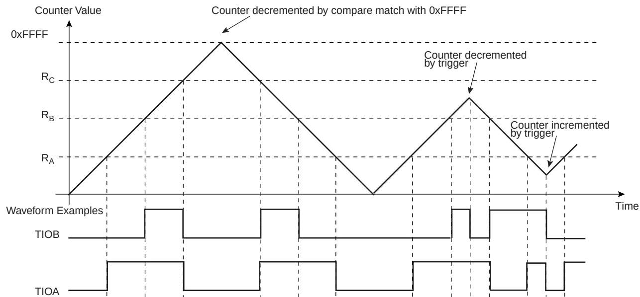
Figure 39-12. WAVSEL = 01 With Trigger
