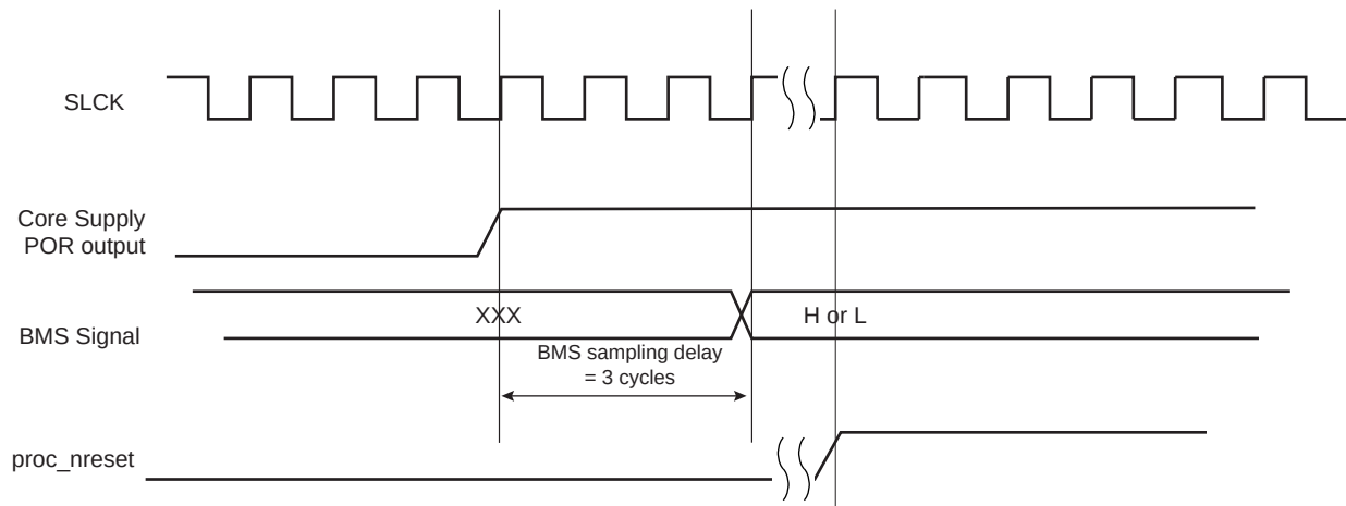
Figure 14-3. BMS Sampling
