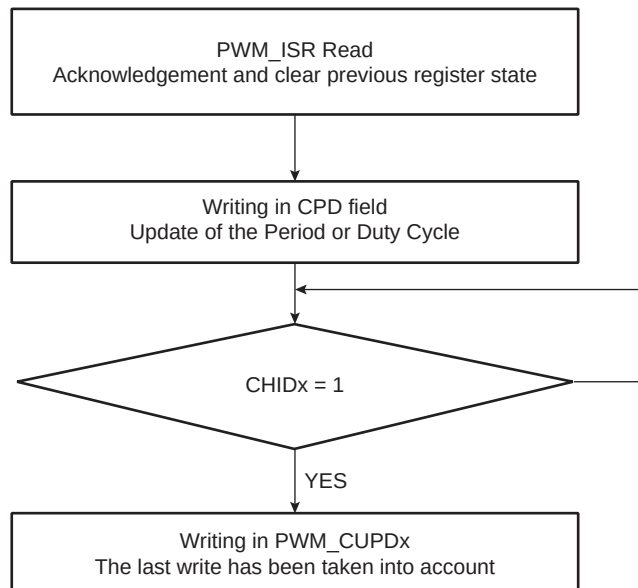
Figure 38-7. Polling Method
