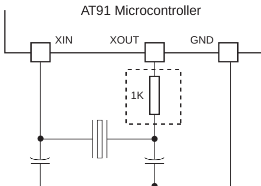
Figure 27-3. Typical Crystal Connection
