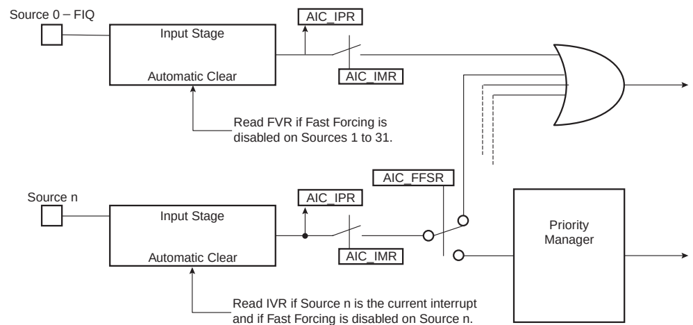
Figure 29-10. Fast Forcing
