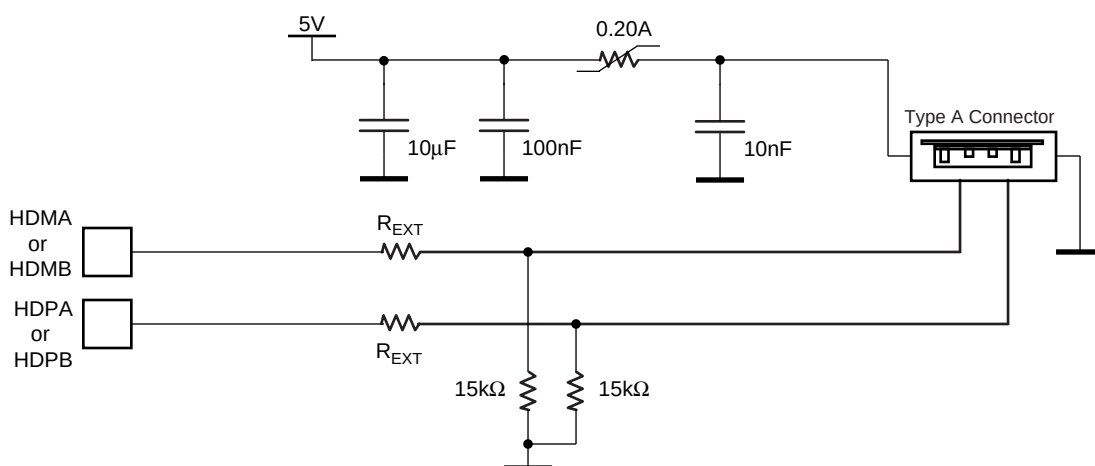
Figure 42-4. Board Schematic to Interface UHP Device Controller
