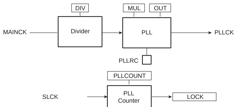
Figure 27-4. Divider and PLL Block Diagram
