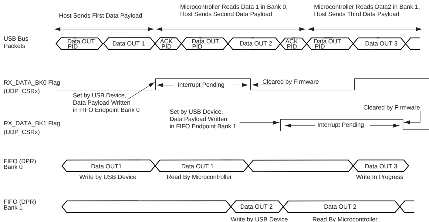
Figure 43-11. Data OUT Transfer for Ping-pong Endpoint
