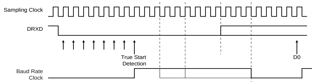
Figure 30-4. Start Bit Detection
