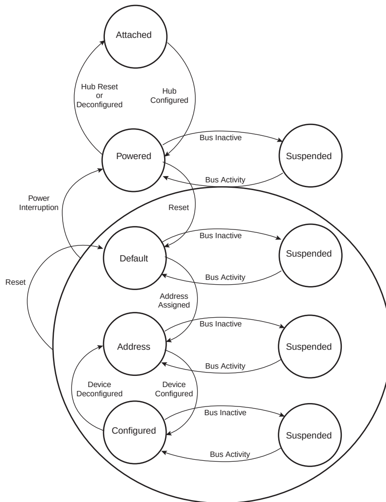
Figure 43-14. USB Device State Diagram
