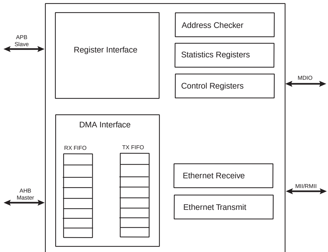
Figure 41-1. EMAC Block Diagram
