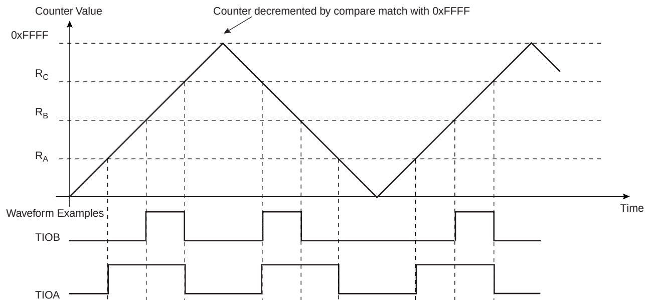
Figure 39-11. WAVSEL = 01 Without Trigger
