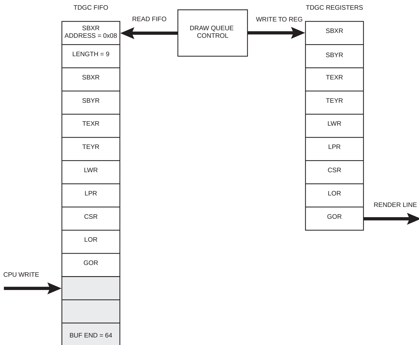
Figure 45-11. Command Queuing
