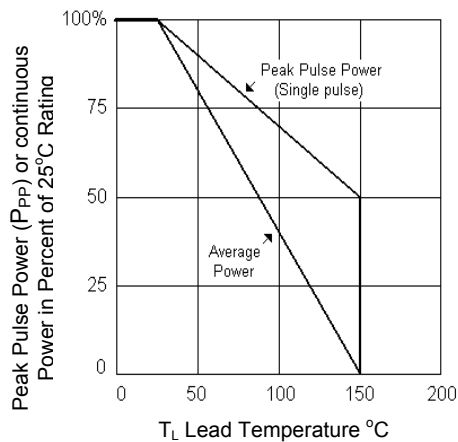
FIGURE 3 - Derating Curve
