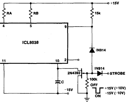
Figure 5: Strobe-Tone Burst Generator.
