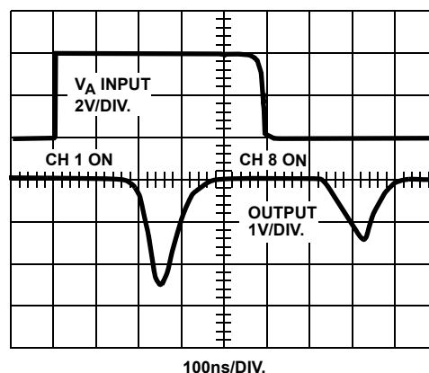
BREAK-BEFORE-MAKE DELAY ( t_{OPEN} )
