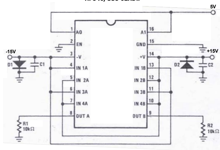
HI-549/883 Cerdip
