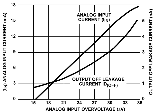
FIGURE 3. ANALOG INPUT OVERVOLTAGE CHARACTERISTICS
