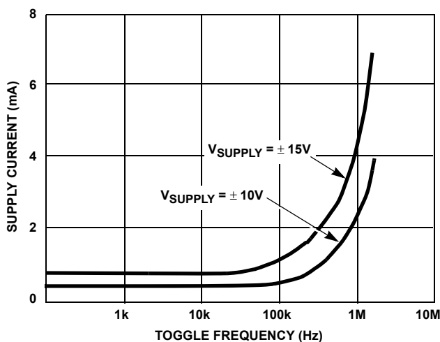
FIGURE 5. SUPPLY CURRENT vs TOGGLE FREQUENCY
