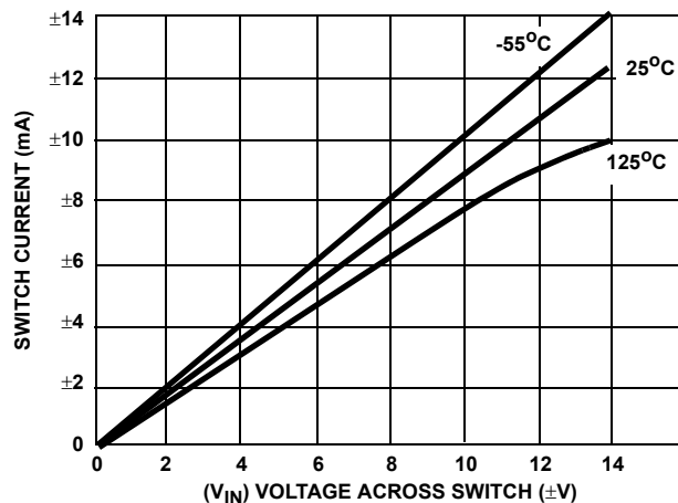
FIGURE 4. ON CHANNEL CURRENT vs VOLTAGE
