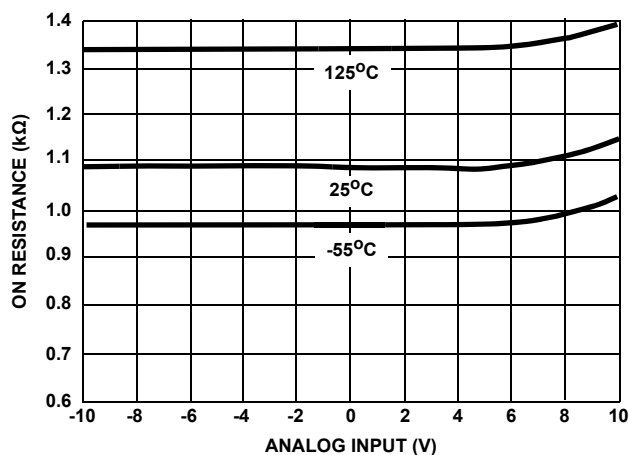
FIGURE 1. ON RESISTANCE vs ANALOG INPUT VOLTAGE
