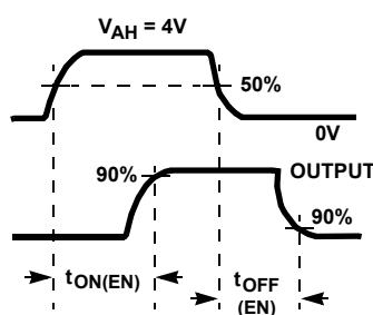
ENABLE DRIVE
