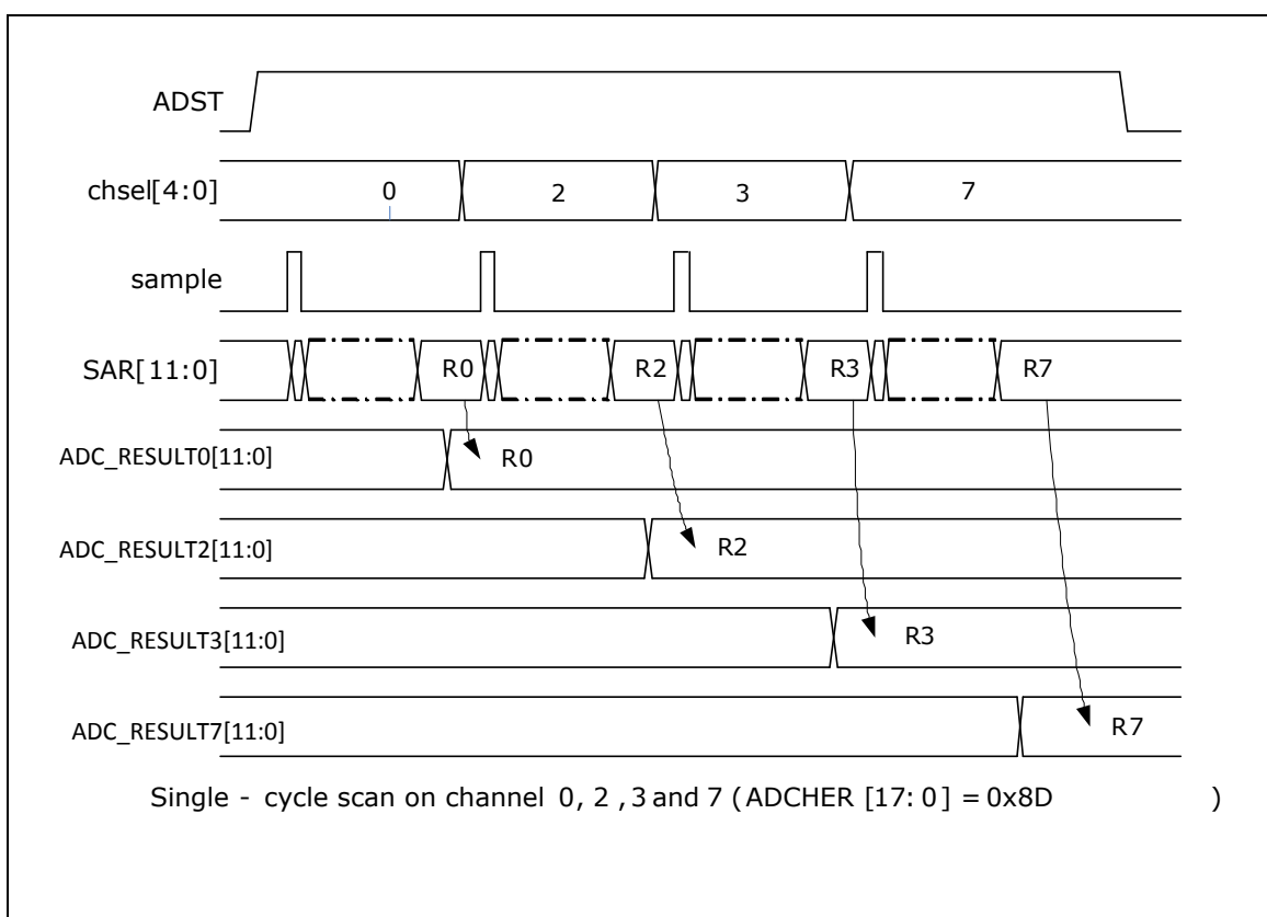
Figure 5-9 ADC Single-cycle Scan on Enabled Channels Timing Diagram
