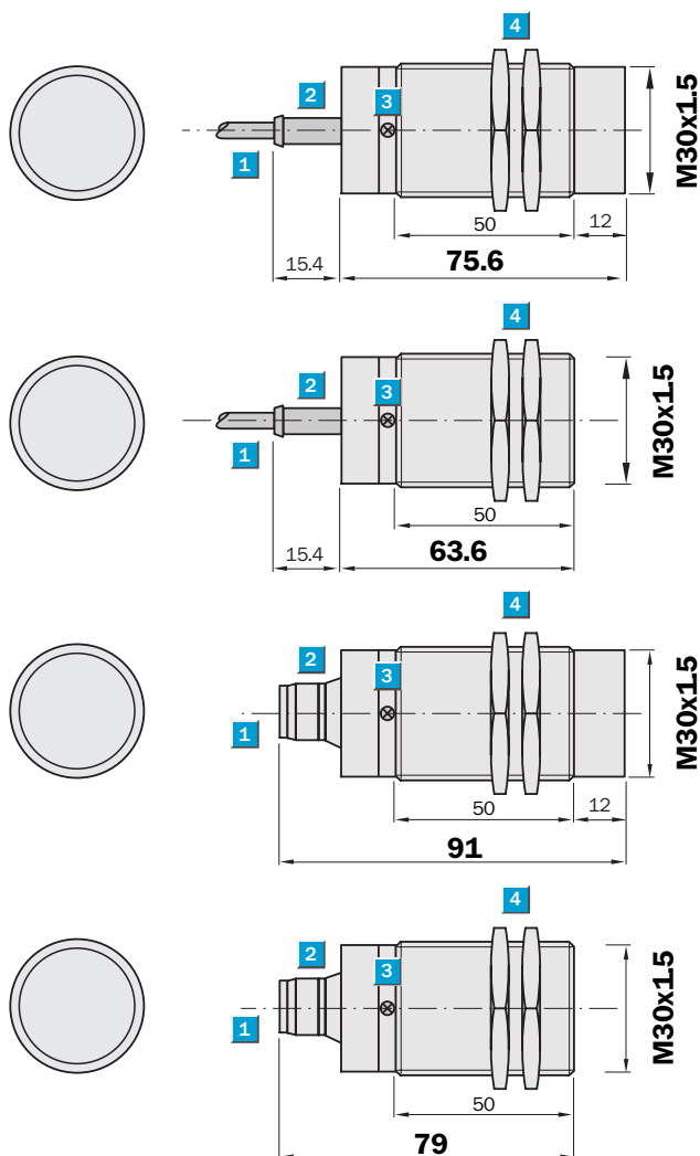
Dimensional drawing
