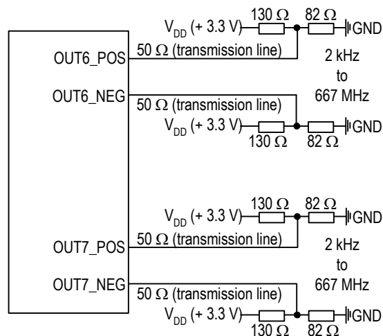
Figure 36. Recommended PECL Output Port Line Termination
