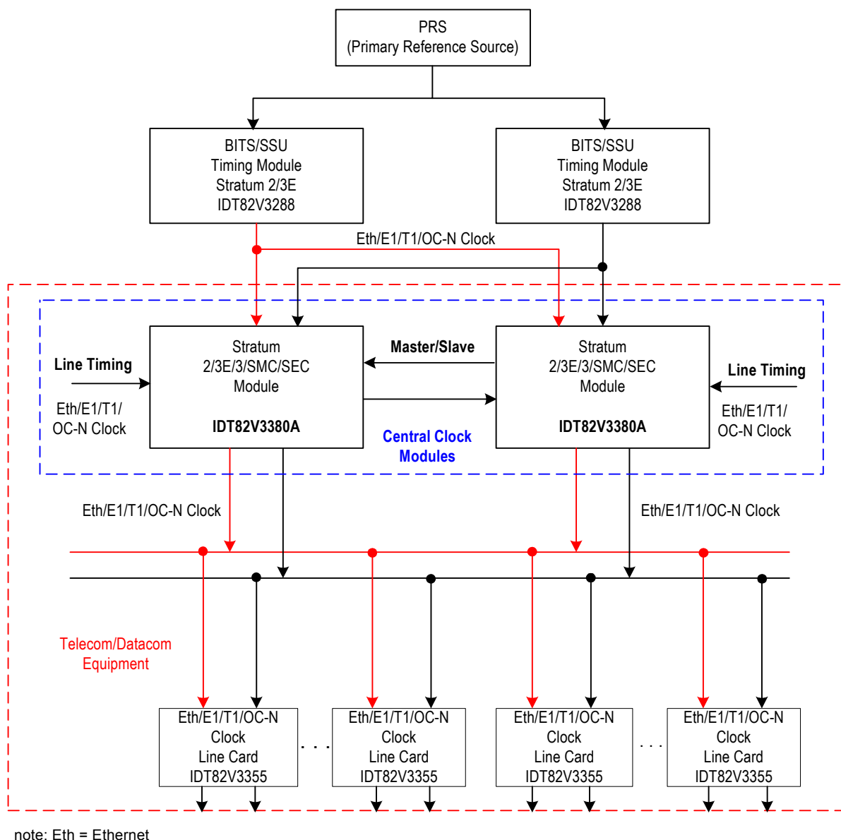
Figure 17. Typical Application
