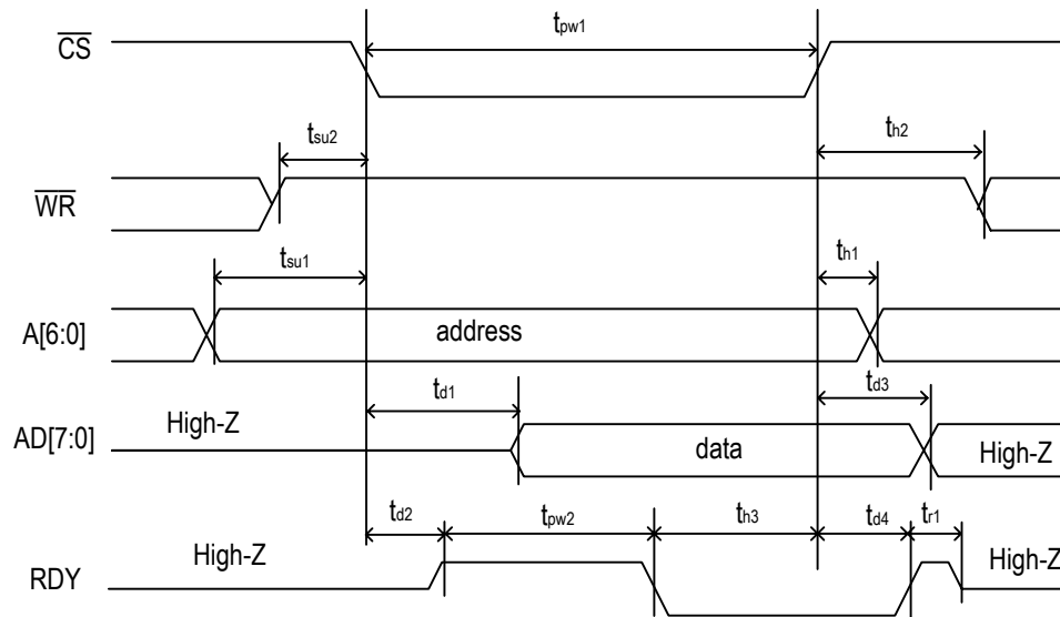
Figure 23. Motorola Read Timing Diagram
