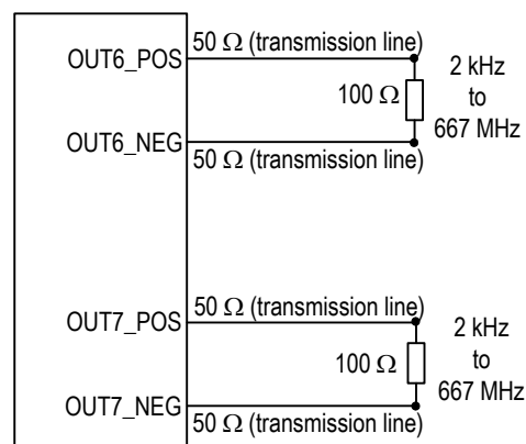
Figure 38. Recommended LVDS Output Port Line Termination
