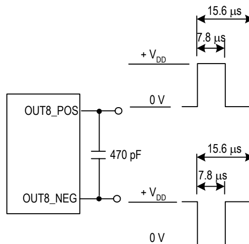
Figure 33. 64 kHz + 8 kHz / 64 kHz + 8 kHz + 0.4 kHz Signal Output Level
