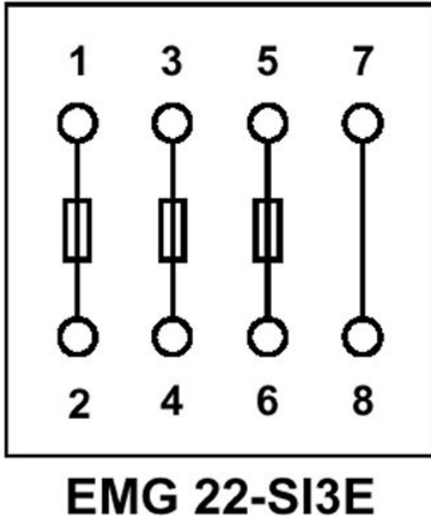
Circuit diagram
