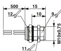
M8 flush-type socket, M10 fastening thread
