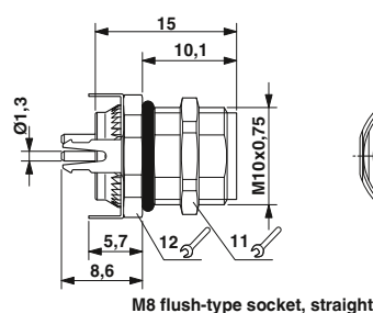
M8 flush-type socket, straight
