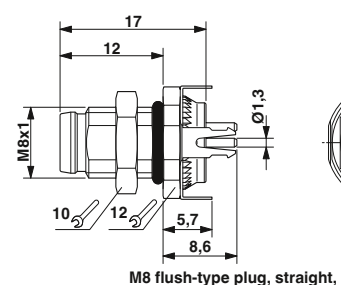
M8 flush-type plug, straight,
