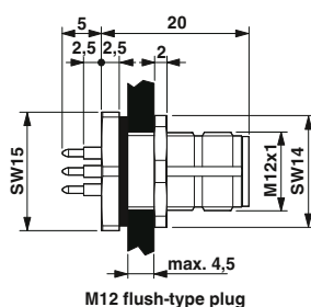
M12 flush-type plug
