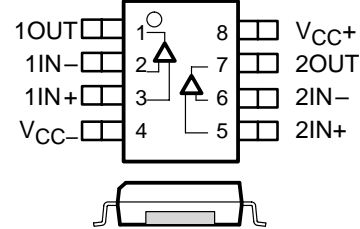
THS4082 D OR DGN PACKAGE (TOP VIEW)
