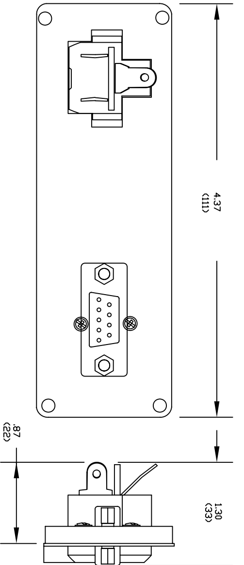
VIEW A (P-03-HX3RO-U66 BACK SIDE)
