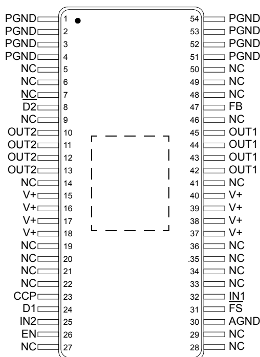
Figure 5. 33887 Pin Connections
