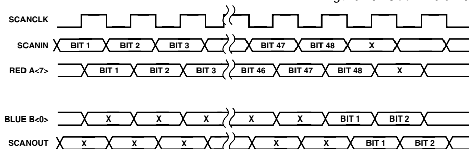
Figure 10. SCAN Timing
