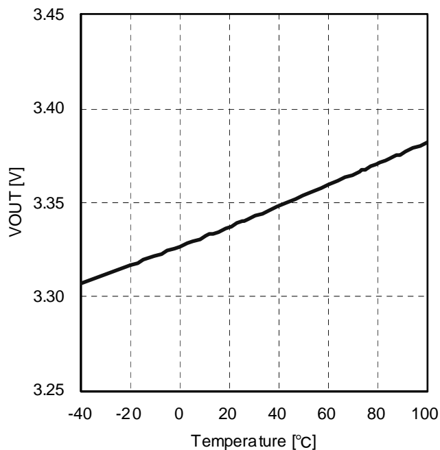
Fig.10 VOUT - Temperature ( V_{\text{IN}}=12\text{V} , V_{\text{OUT}}=3.3\text{V} , L=3.3\mu\text{H} , I_{\text{out}}=0\text{A} )
