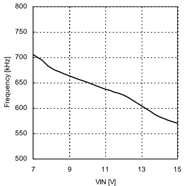
Fig.11 Frequency - VIN ( V_{\text{IN}}=12\text{V} , V_{\text{OUT}}=3.3\text{V} , L=3.3\mu\text{H} , I_{\text{out}}=0\text{A} )
