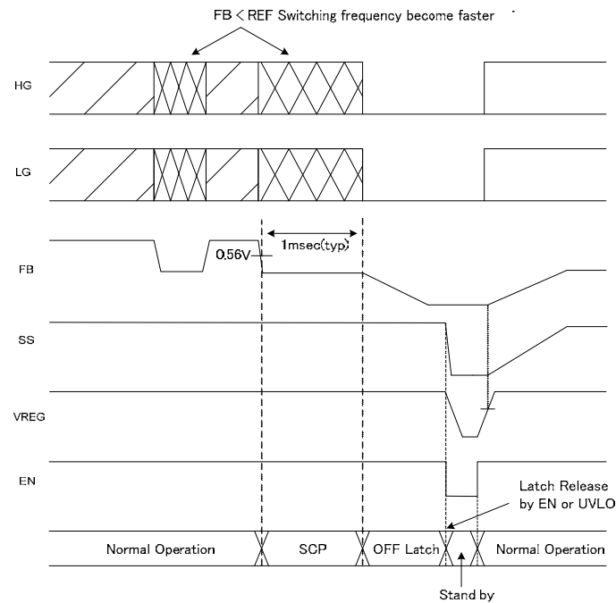
Fig.20 SCP Timing Chart
