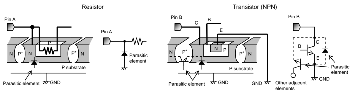
Fig.29 Example of IC structure
