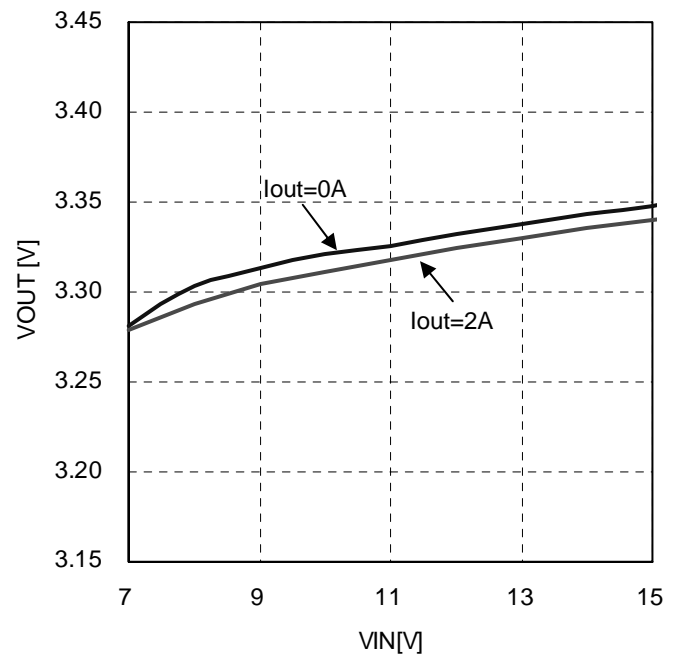
Fig.9 VOUT Line Regulation ( V_{\text{OUT}}=3.3\text{V} , L=3.3\mu\text{H} , I_{\text{out}}=0\text{A} / 2\text{A} )
