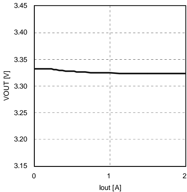
Fig.8 VOUT Load Regulation ( V_{\text{IN}}=12\text{V} , V_{\text{OUT}}=3.3\text{V} , L=3.3\mu\text{H} )
